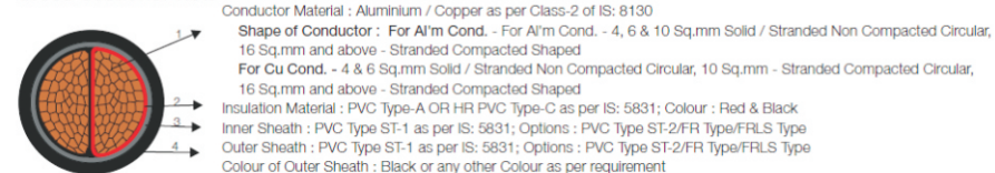
UNARMoured CABLES Cross-sectional view
