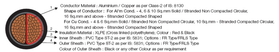
UNARMOURED CABLE
