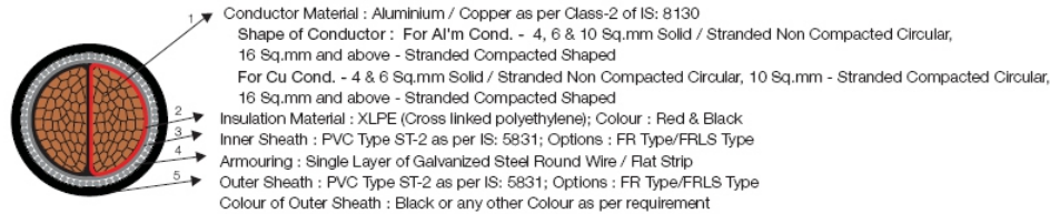
ARMOURFD CABIE
